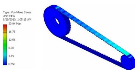
Figure 17 Von-mises stress at M = 7.5 N-m.
