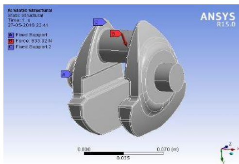
Figure 15 Model of crankshaft.
