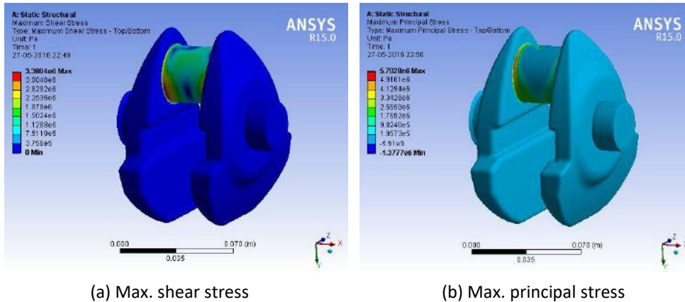
Figure 16 Stresses on crankshaft for static analysis.
